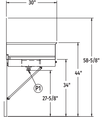
SL30 Side Loader Right to Left Operation
