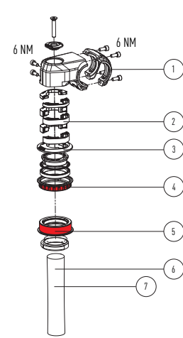
COCKPIT WITH BLOCK LOCK
