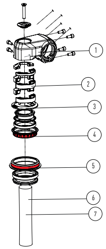
COCKPIT 1.8 WITHOUT BLOCK LOCK
