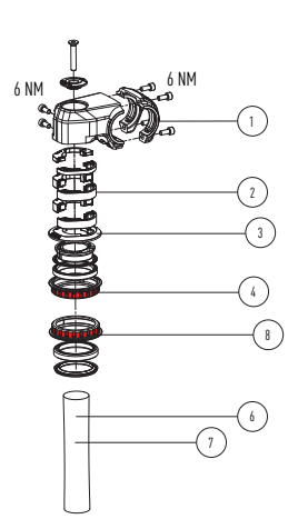
COCKPIT WITHOUT BLOCK LOCK
