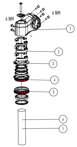
COCKPIT 30° WITHOUT BLOCK LOCK
