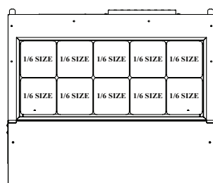
PAN LAYOUT
