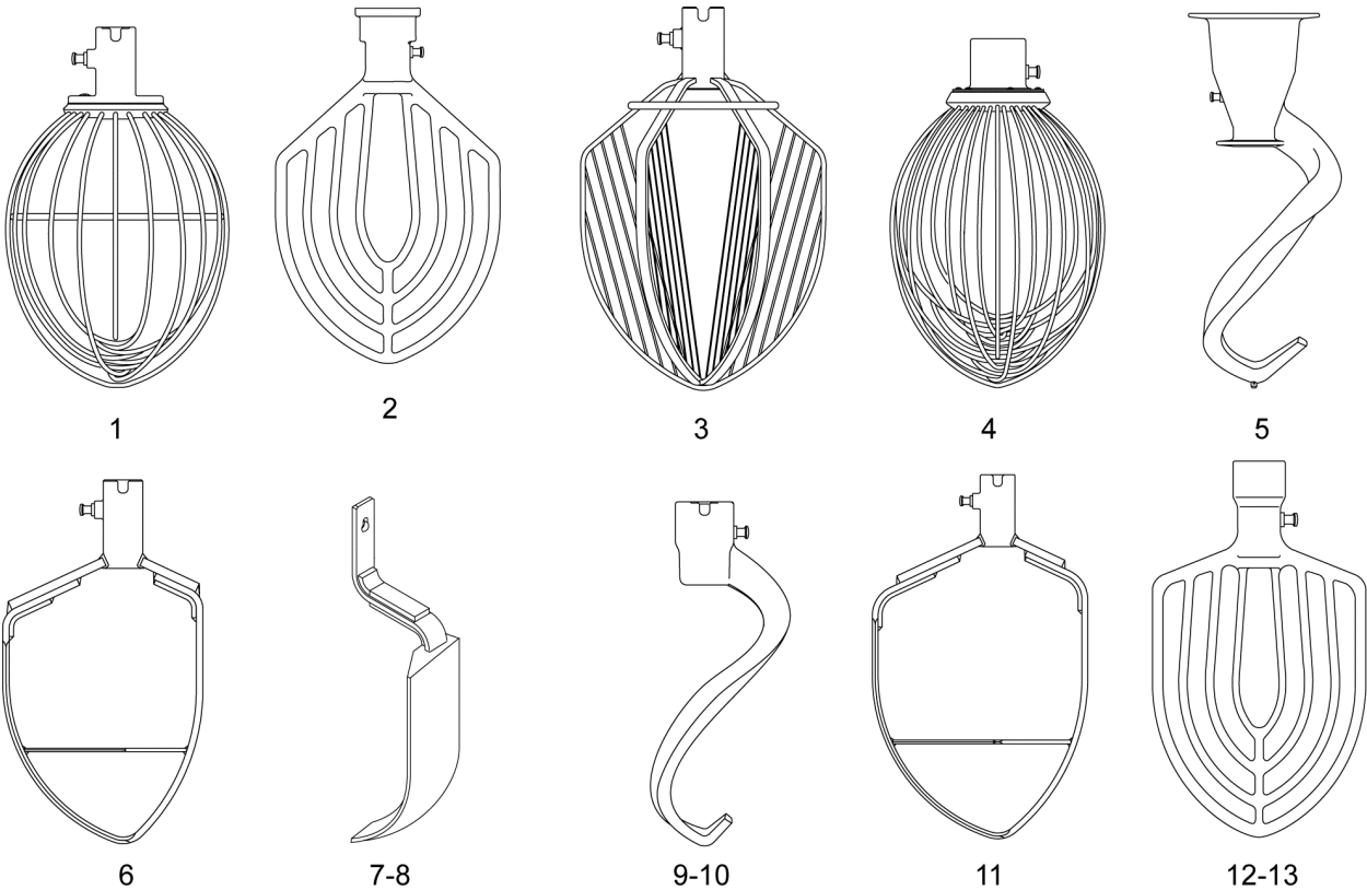
80-QUART AGITATORS
