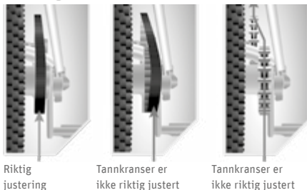
Fig. 108 Rette inn reim ©Gates
