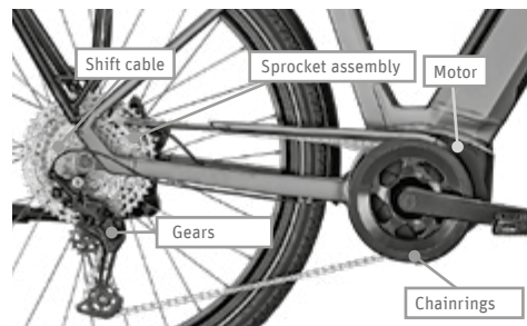
Fig. 62 Mechanical derailler
