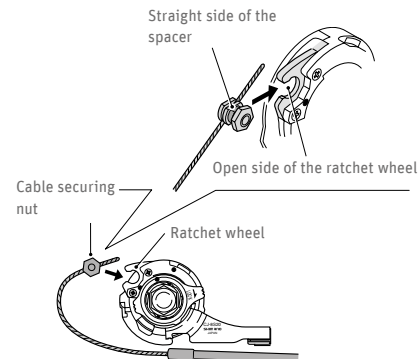
Fig. 138 Mounting the cable ©Shimano
