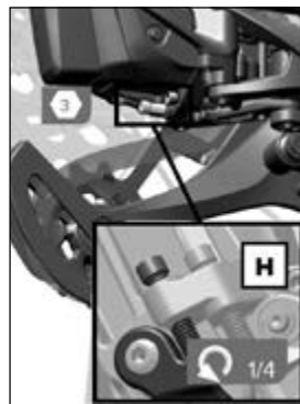
Sl. 92 Vijak prislona H ©Sram
