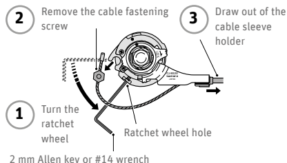
Fig. 131 Tip for removing the cable sleeve ©Shimano
