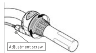
Fig. 100 Shimano standard twist grip ©Shimano
