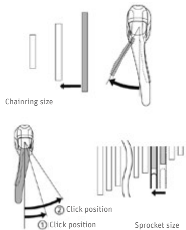
Fig. 72 Shifting to a lower gear ©Shimano
