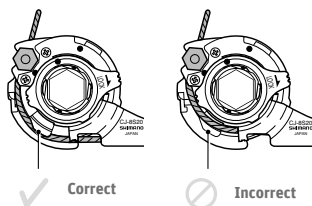
Fig. 141 Checking the cable arrangement ©Shimano
