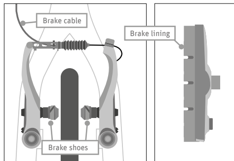
Fig. 51 Rim brakes
