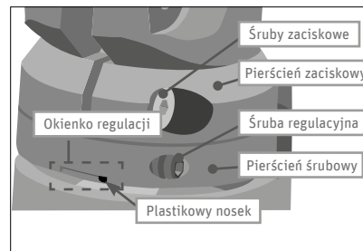
Rys. 37 Stery Ahead II
