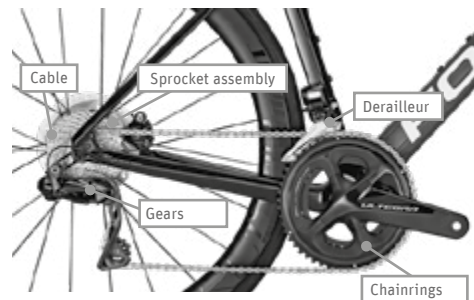
Fig. 63 Electronic derailler
