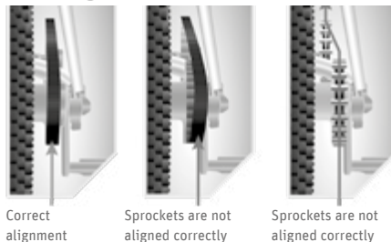
Fig. 108 Aligning the belt ©Gates
