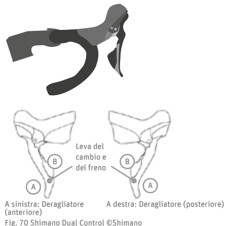
Fig. 70 Shimano Dual Control ©Shimano
