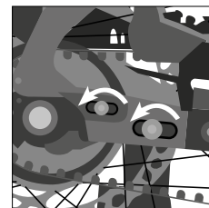
Fig. 109 Loosening the screws
