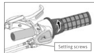
Fig. 101 Shifting to a lower gear ©Shimano
