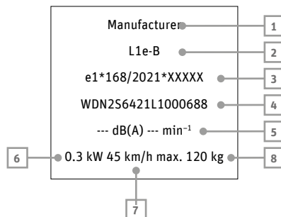
Fig. 10 Manufacturer's type plate
