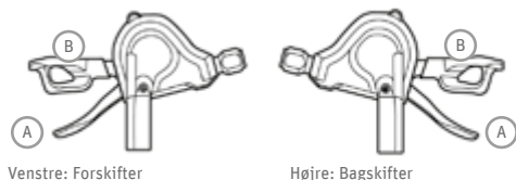
Fig. 67 Shimano-standardskiftegreb ©Shimano
