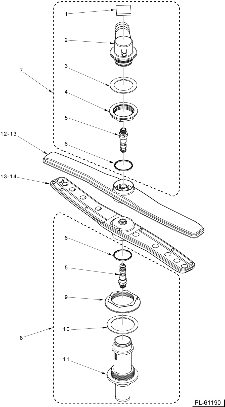
WASH ARM ASSEMBLY
