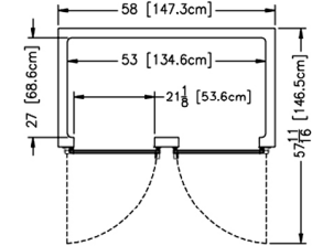
Plan - R/AHT232WUT
