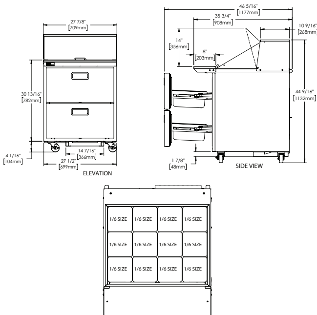
PAN LAYOUT
