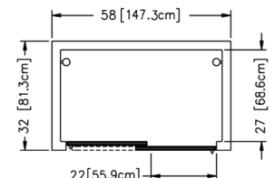
Plan - RHT232WUTSL
