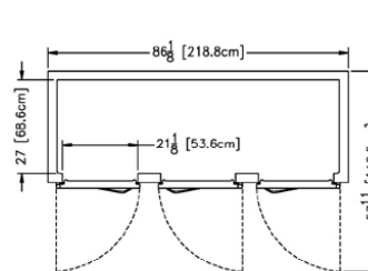
Plan - R/AHF332W
