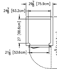
Plan - R/AHF132W
