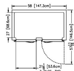
Plan - R/AHF232W
